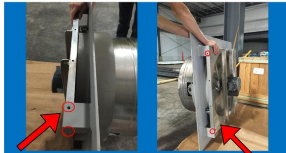
IDENTIFY ATTACHMENT POINTS & SECURE FAN TO MOUNTING PLATE
